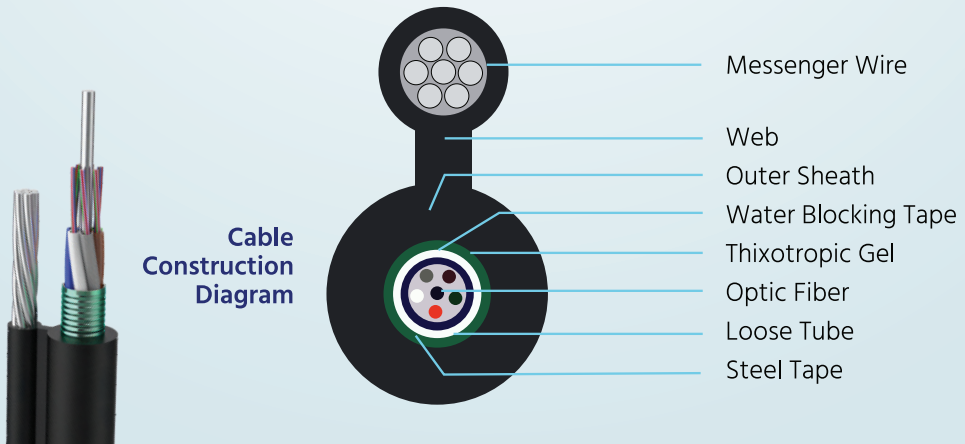
6F Aerial Cable (Fig-8) with Cross Sectional Diagram
