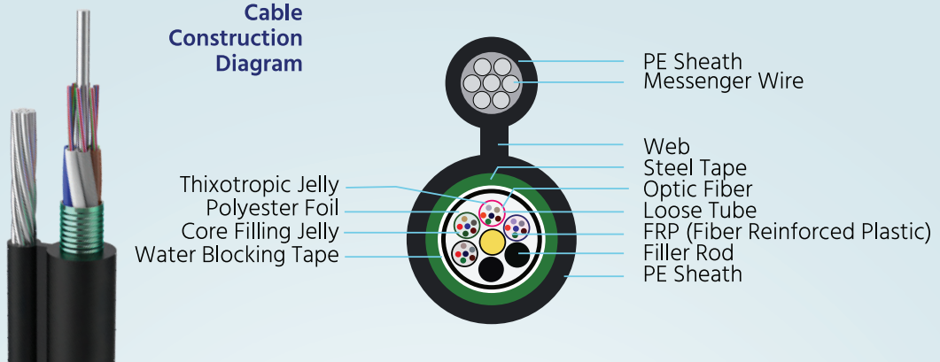
12F-24F Fig-8 Aerial Cross Sectional Diagram
