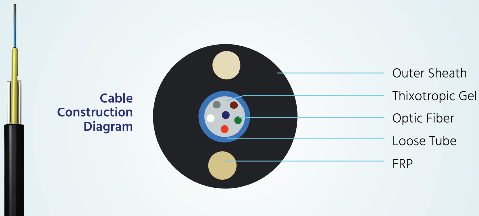
6F Non-armoured with Cross Sectional Diagram
