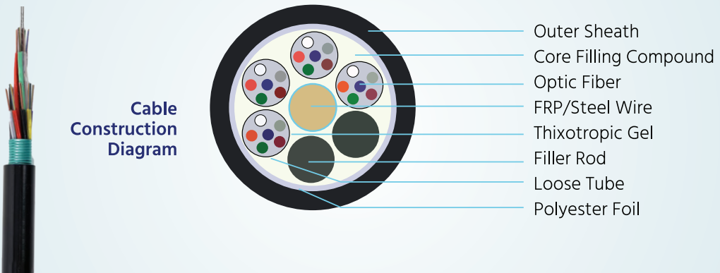
12F-144F Armoured Cable Cross Sectional Diagram
