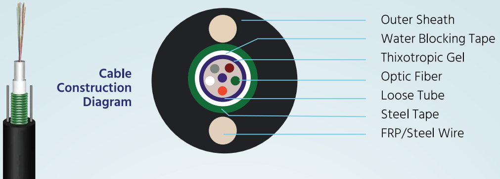
6F Armoured Cable with Cross Sectional Diagram
