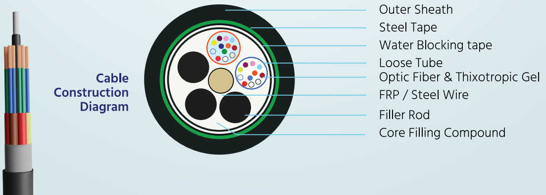
12F-144F Non-armoured Cable Cross Sectional Diagram
